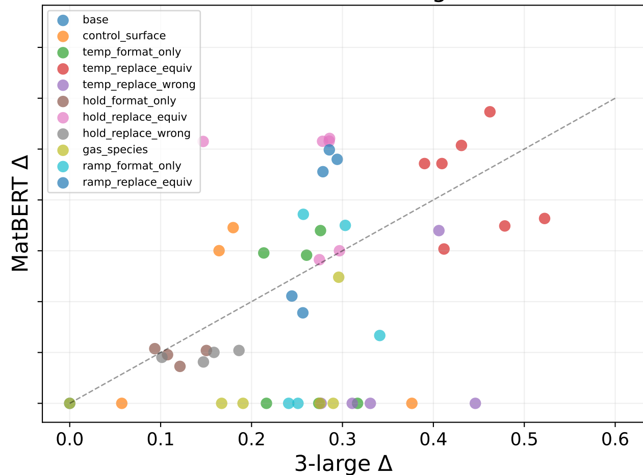
MatBERT vs 3-large
