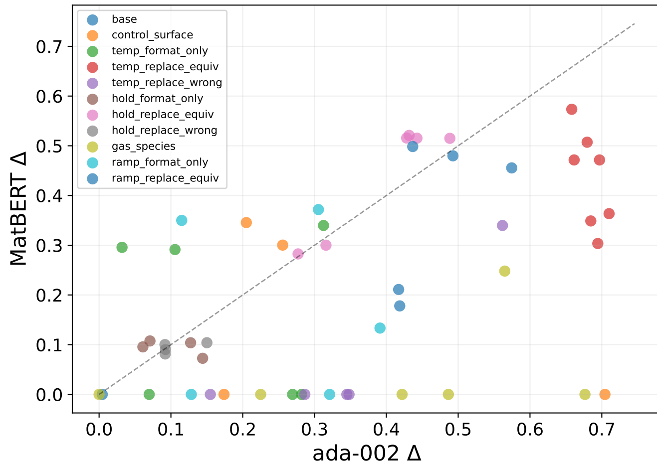
MatBERT vs ada-002
